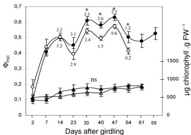
Figure 5. Quantum yield efficiency of photosystem II ( \Phi_{PSII} , \circ , \bullet ) and chlorophyll concentration ( \Delta , \blacktriangle ) of young leaves of multiple-flowering leafy shoots of trunk girdled (filled symbols) and ungirdled (open symbols) 'Loretina' mandarin. Data are means \pm SE of 25 leaves. Numbers in the figure are means of the number of fruitlets per shoot. Significant differences ( P \leq 0.05 ) between treatments are denoted by an asterisk (*).
