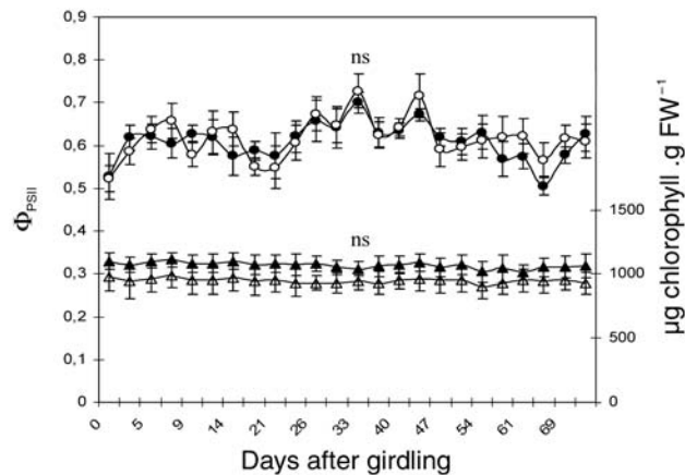
Figure 4. Quantum yield efficiency of photosystem II ( \Phi_{PSII} , \circ , \bullet ) and chlorophyll concentration ( \Delta , \blacktriangle ) of mature leaves of trunk girdled (filled symbols) and ungirdled (open symbols) 'Loretina' mandarin trees. Data are means \pm SE of 25 leaves. None of the treatment differences were significant at P \leq 0.05 (ns = not significant).
