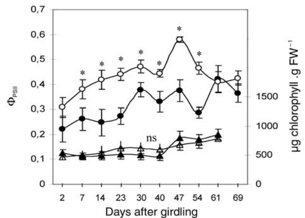
Figure 6. Quantum yield efficiency of photosystem II ( \Phi_{PSII} , \circ , \bullet ) and chlorophyll concentration ( \Delta , \blacktriangle ) of young leaves of vegetative shoots of trunk girdled (filled symbols) and ungirdled (open symbols) 'Loretina' mandarin. Data are mean \pm SE of 25 leaves. Significant differences ( P \leq 0.05 ) between treatments are denoted by an asterisk (*).
